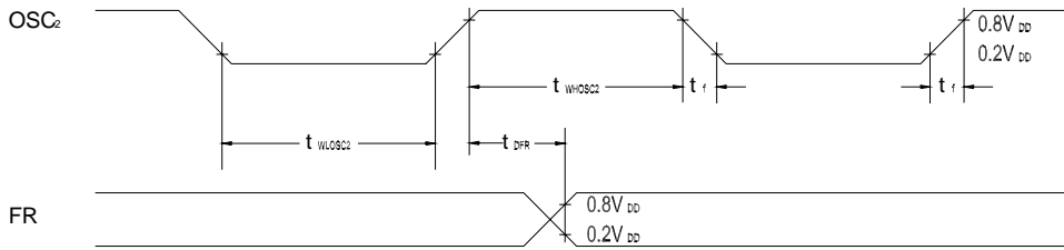
Display control timing characteristics
