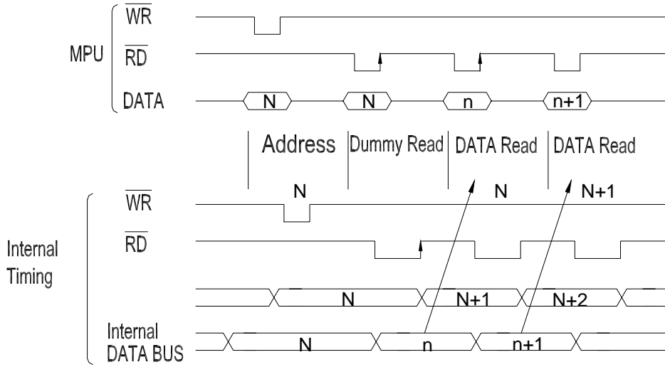
MPU Interface Timing
